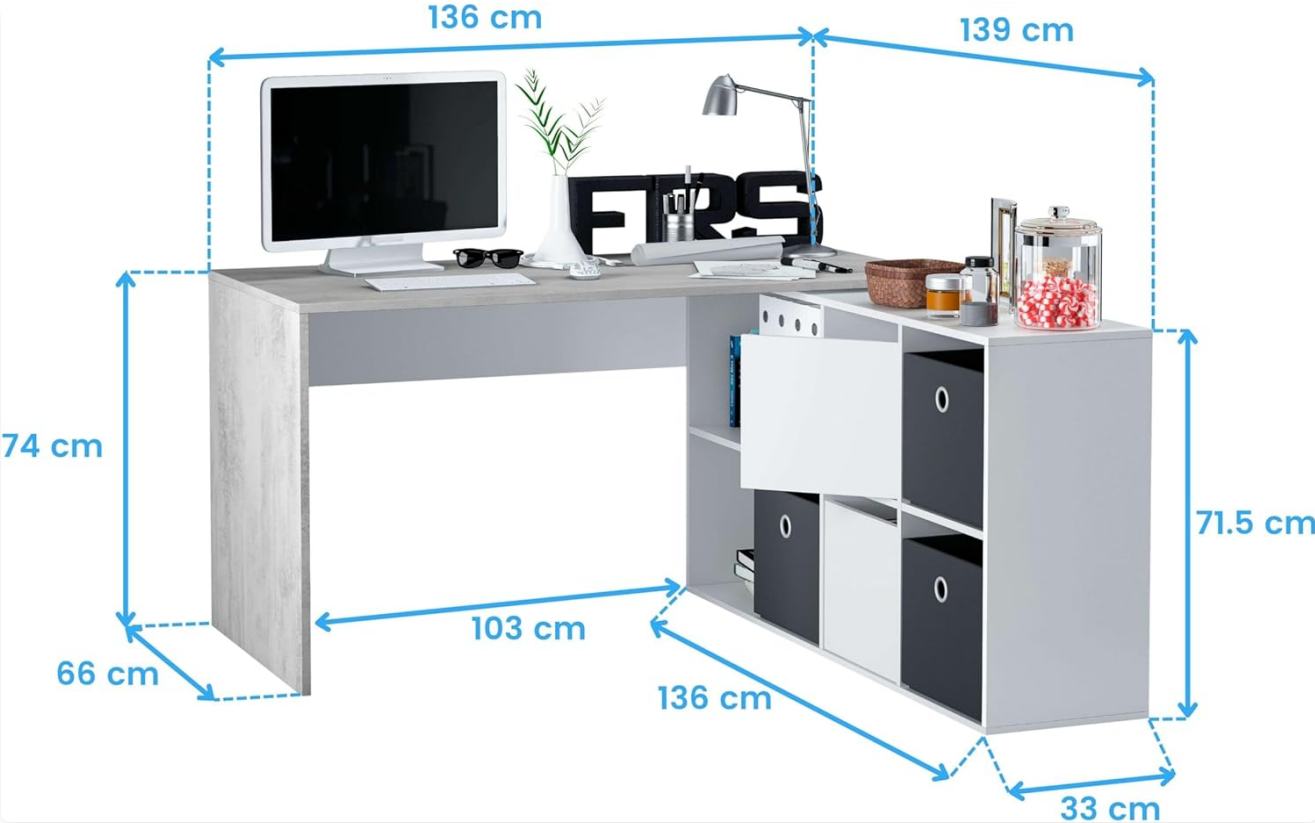
Image 7.1: Detailed dimensions of the desk in an extended configuration.
