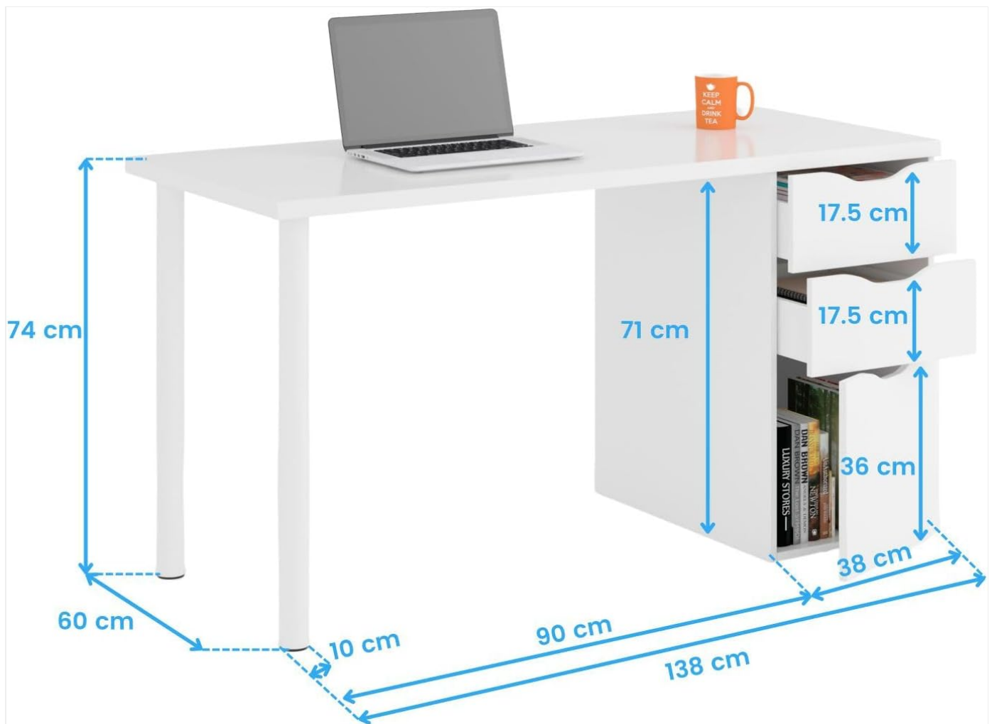
Image 3: A detailed diagram illustrating the dimensions of the Habitdesign Athena desk, including overall width (138 cm), depth (60 cm), height (74 cm), and internal storage measurements.
