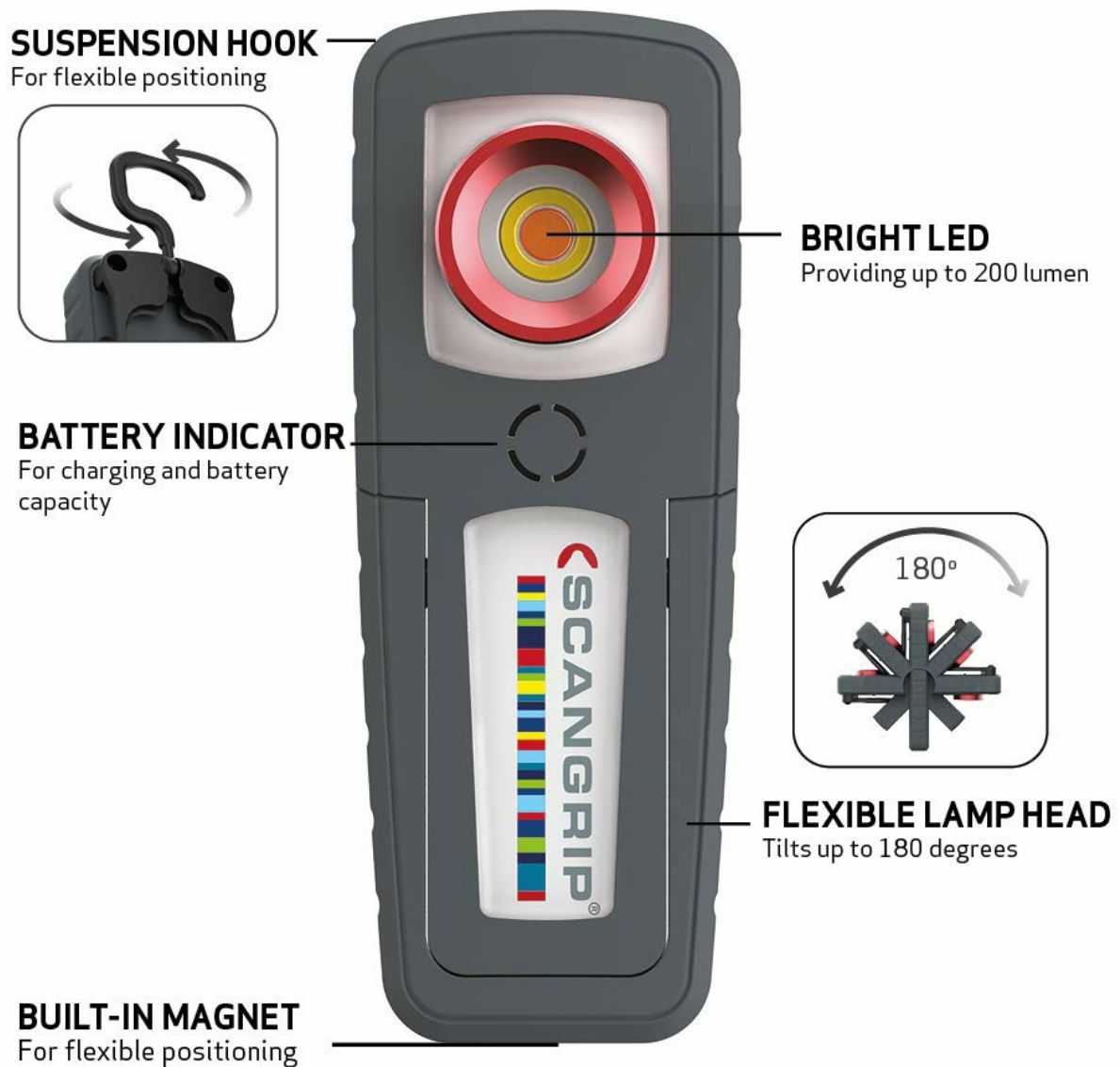
Figure 2: Key features of the SCANGRIP MINIMATCH, including the battery indicator.
