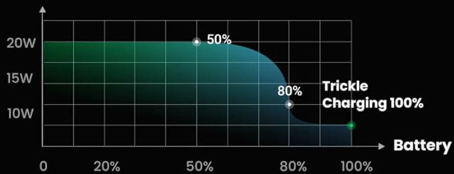
Output Power
