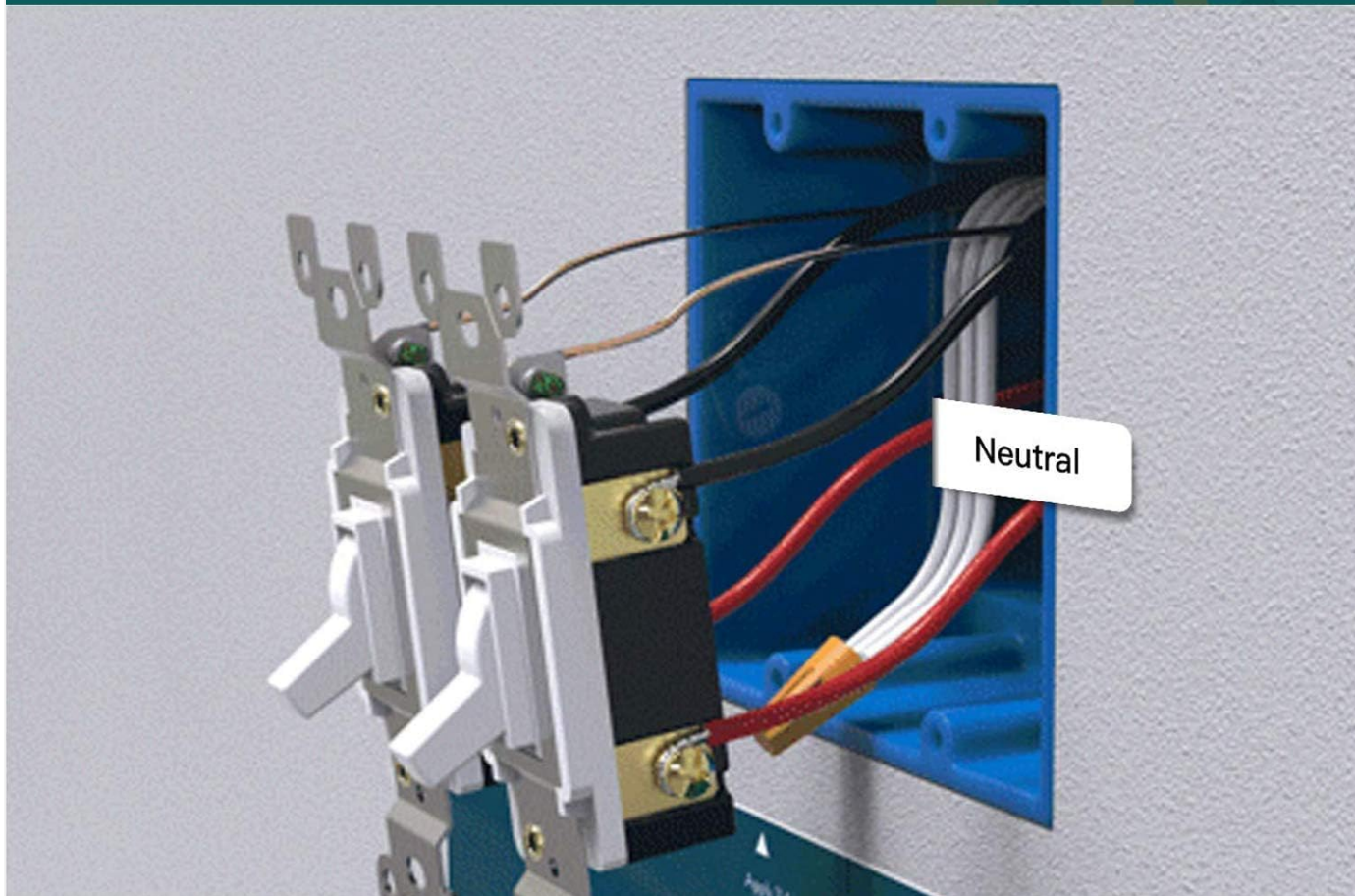
Image: An illustration showing what a neutral wire typically looks like inside a switch box, usually white and bundled.
