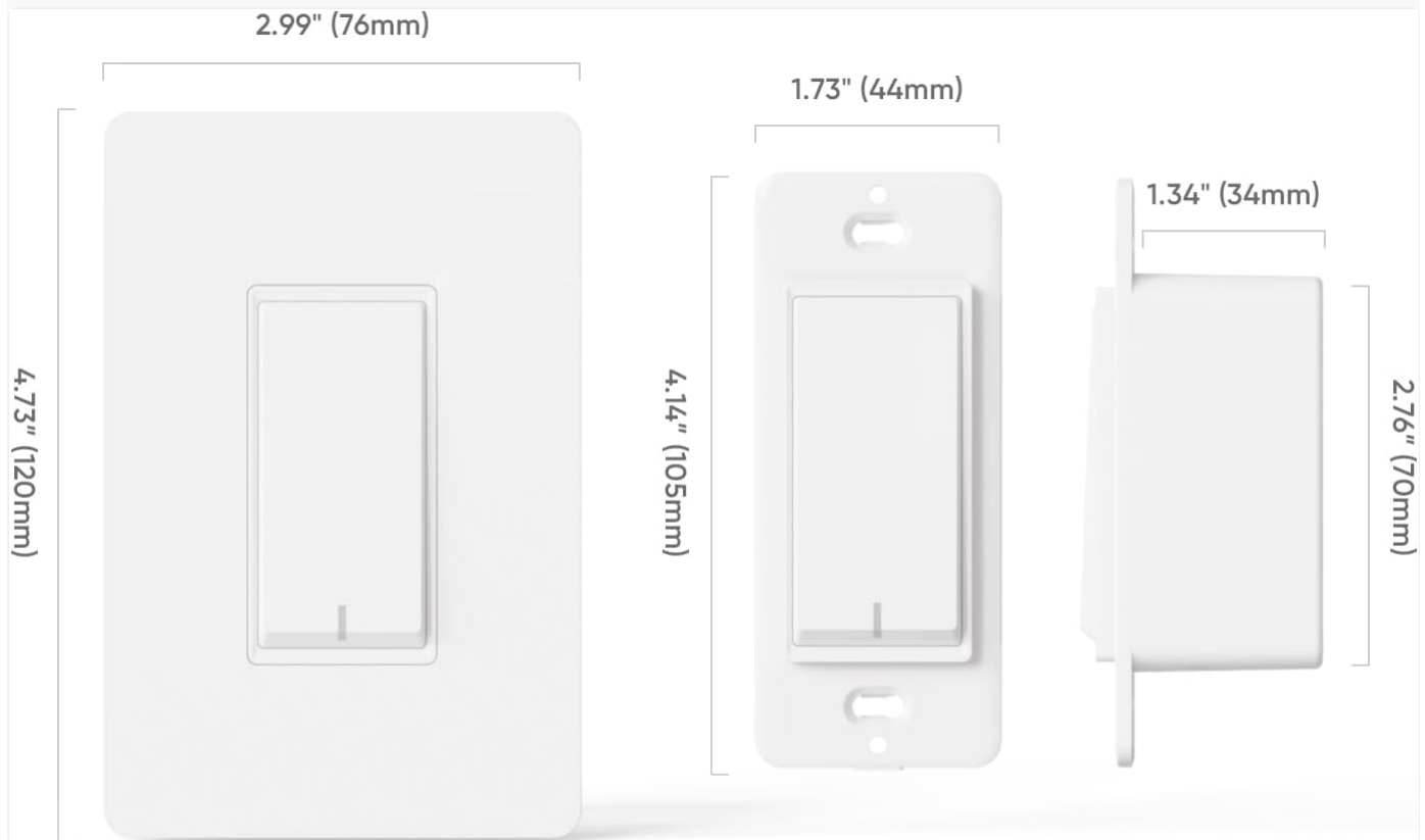
Image: Detailed dimensions of the smart light switch and its wallplate, showing measurements in inches and millimeters.
