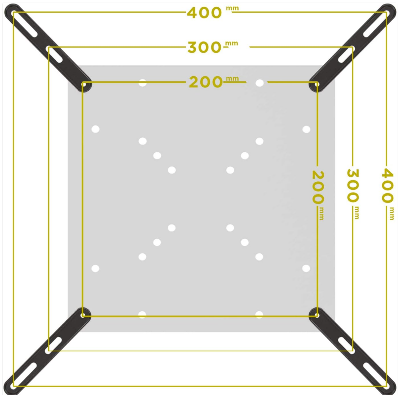
Figure 4.2: VESA Pattern Extension (200mm to 300mm/400mm)
