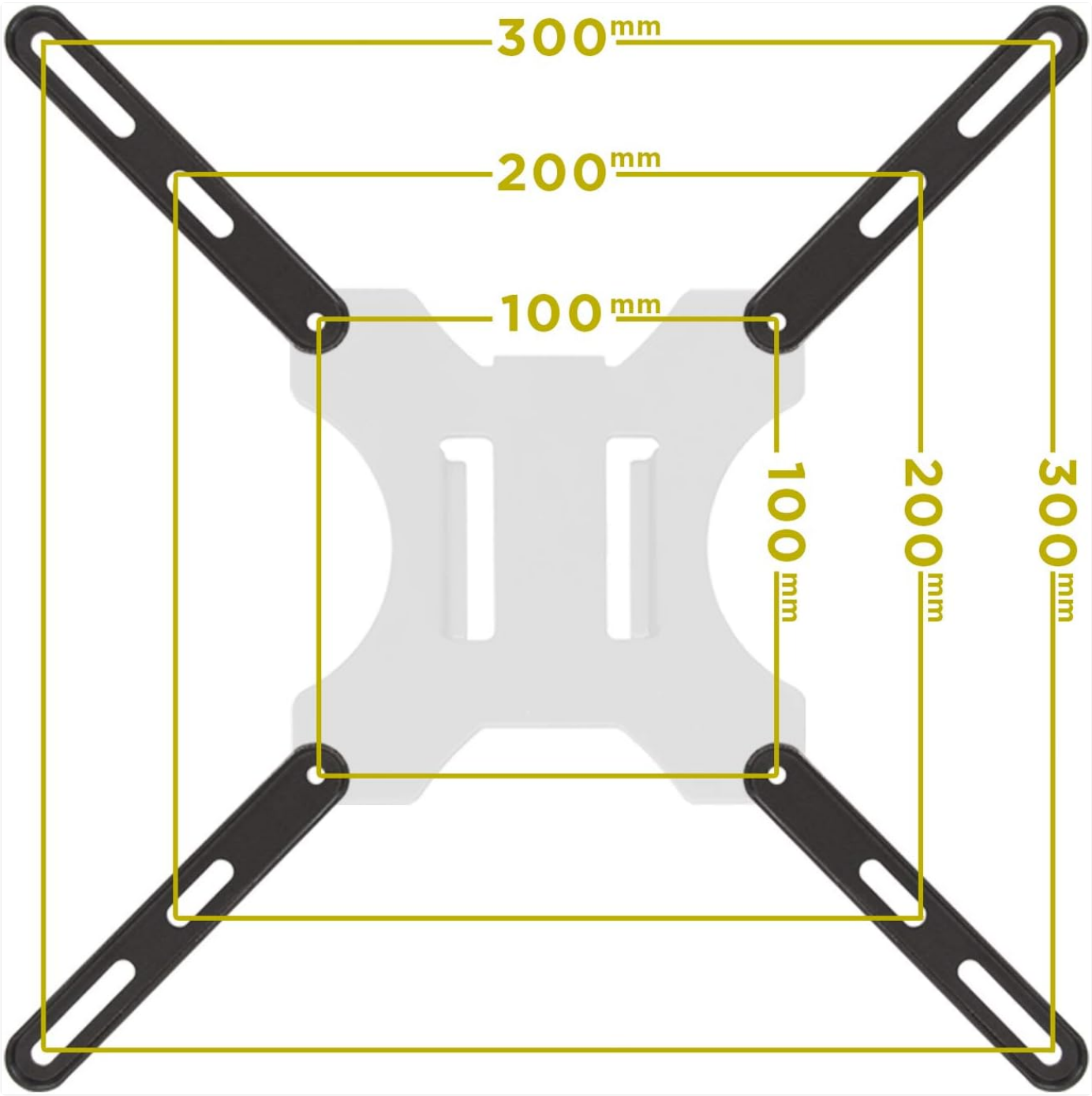
Figure 4.1: VESA Pattern Extension (100mm to 200mm/300mm)
