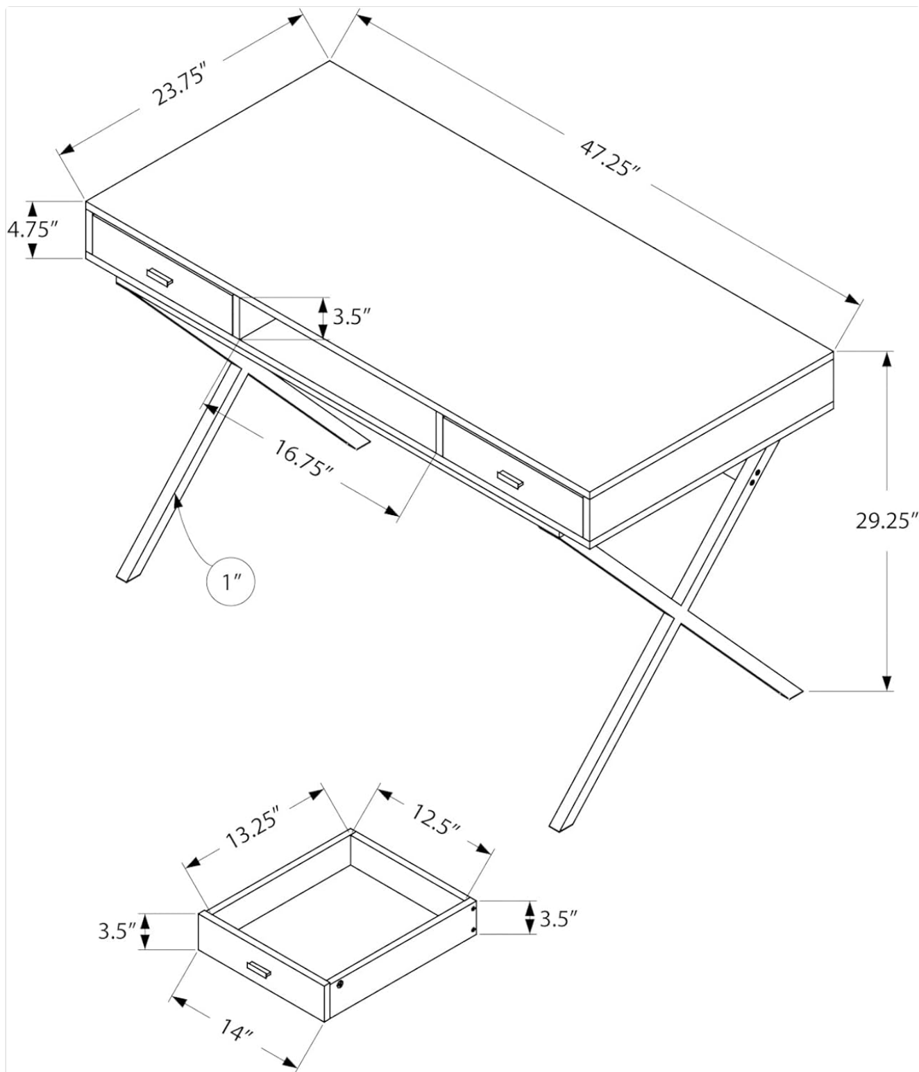
Figure 2: Desk Dimensions
