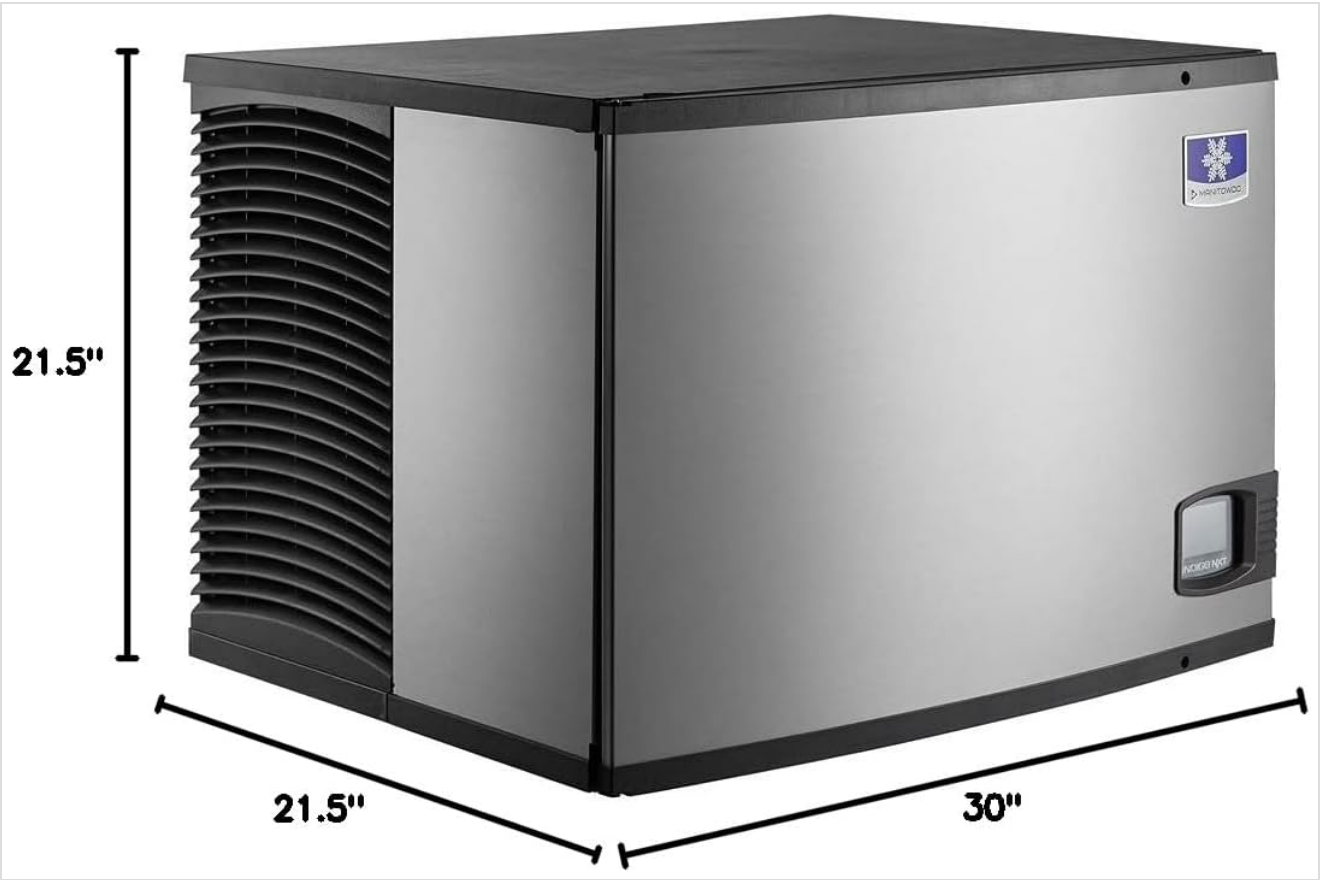
Figure 9: Diagram illustrating the dimensions of the Manitowoc IYT0450A ice machine.
