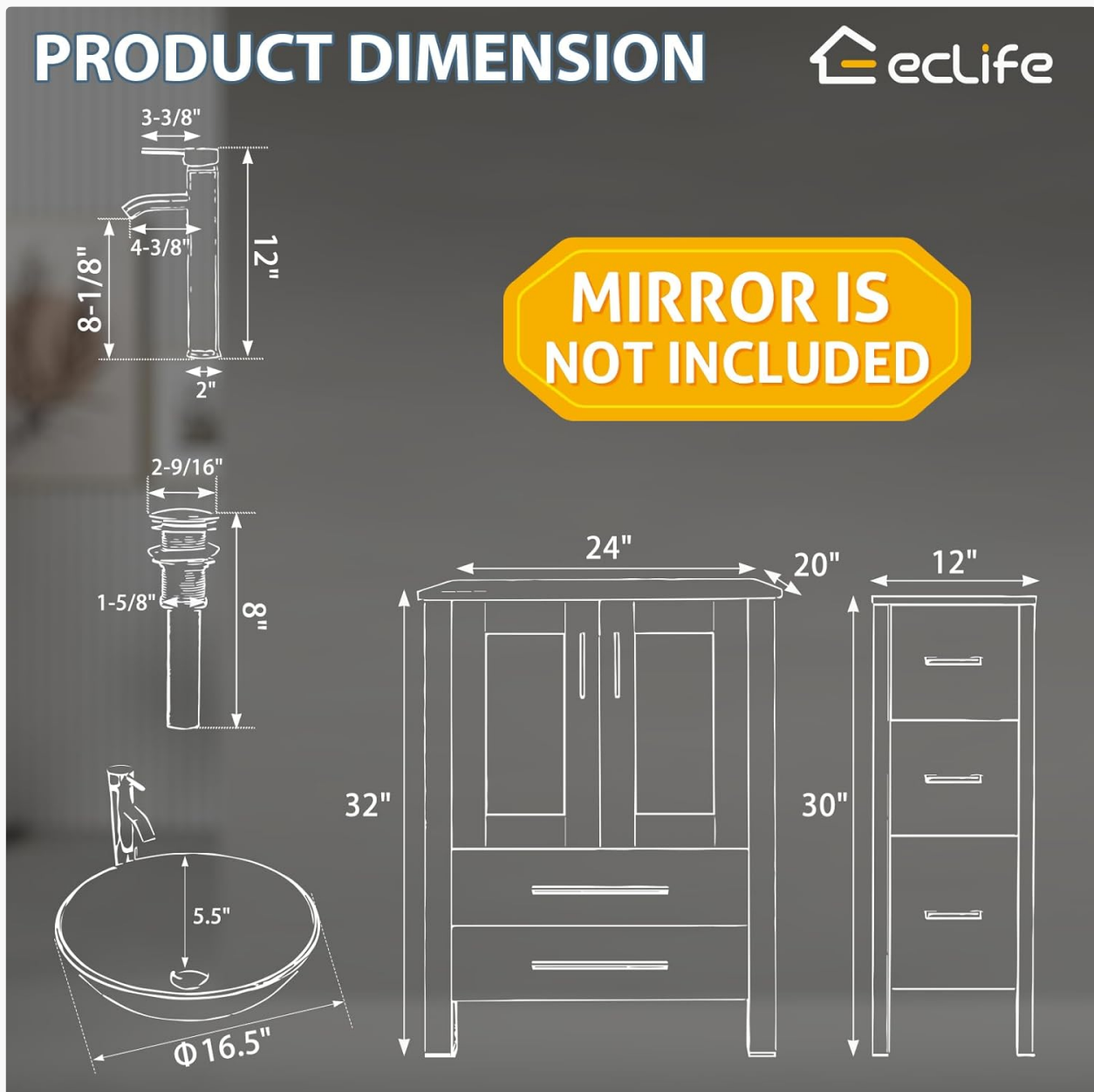
Figure 4.1: Product dimensions for the vanity, sink, and faucet. Ensure these dimensions fit your space before installation.
