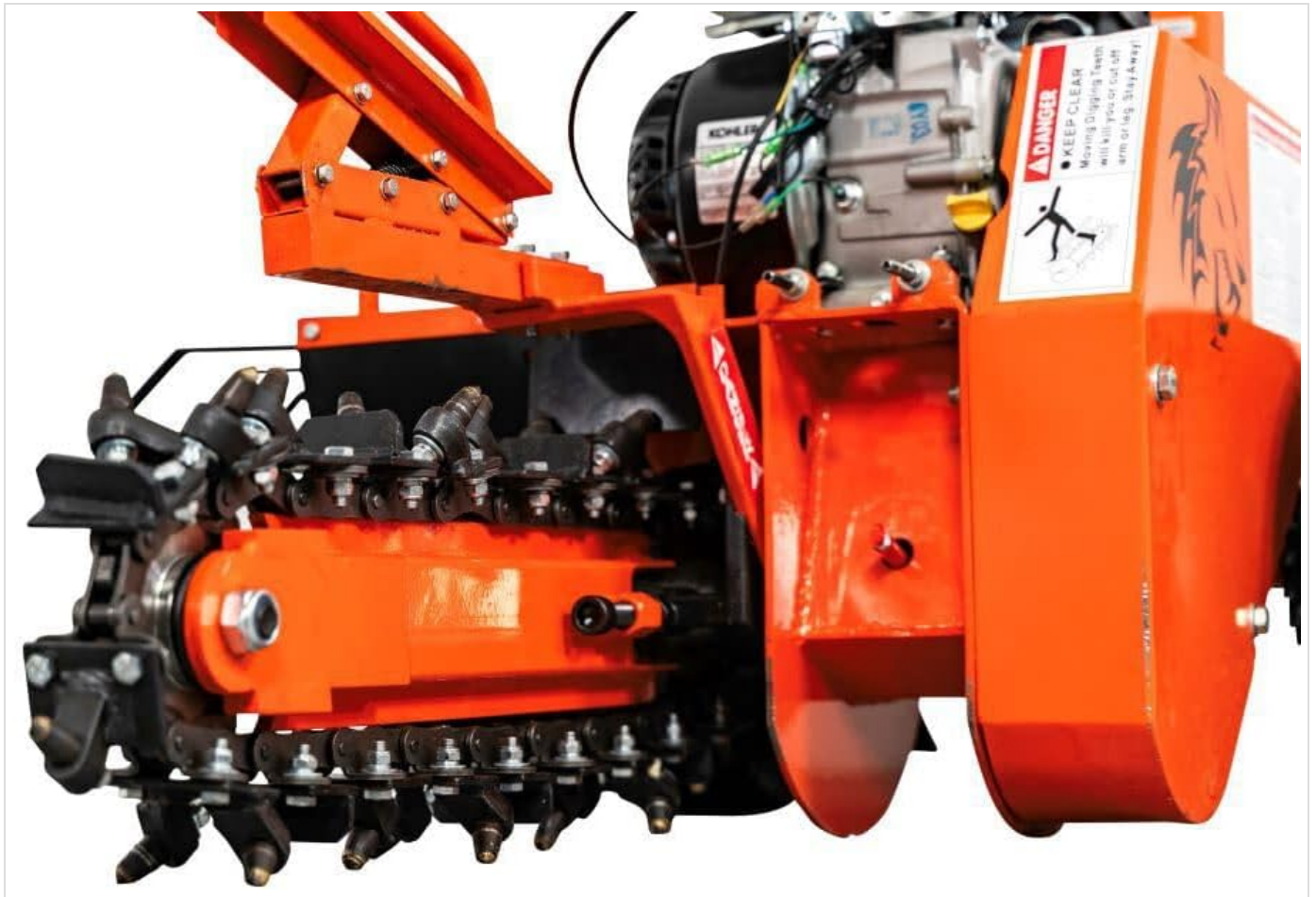
Figure 4: Detailed view of the high-pressure sintered Tungsten Carbide quick-change cutters on the trenching chain.
