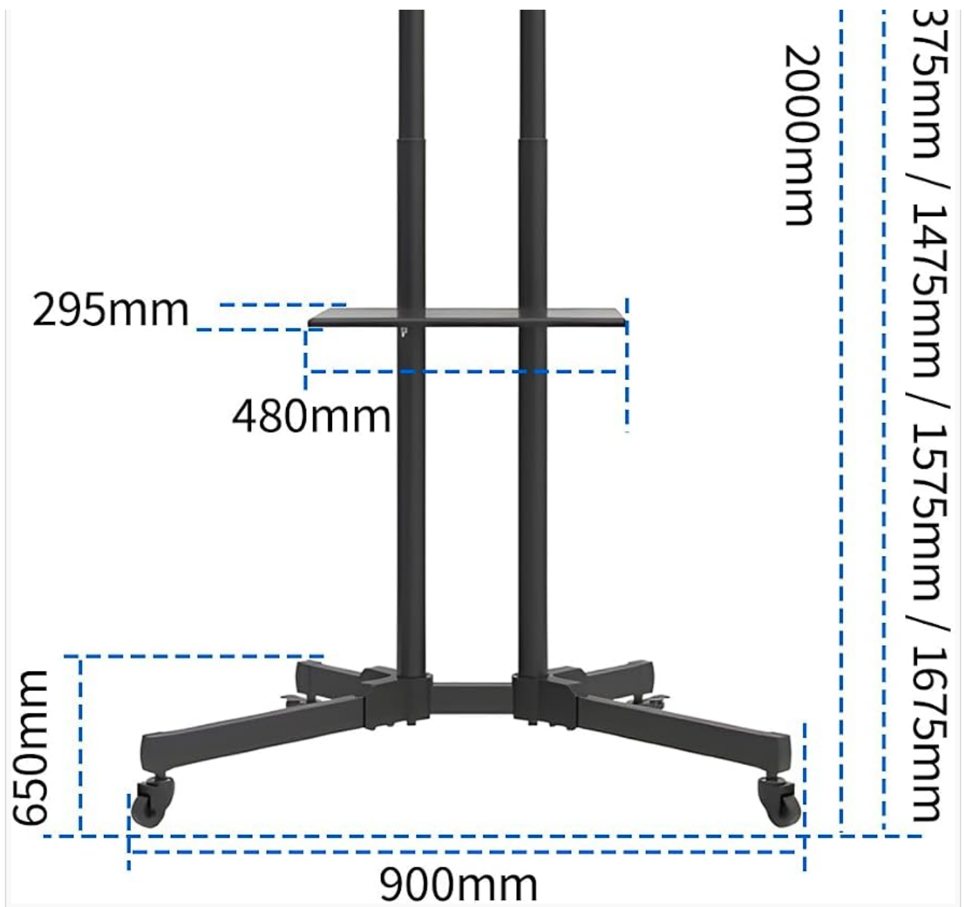
Image: Detailed diagram showing the dimensions of the JAPANNEXT JN-3275-JRSA mobile TV stand.
