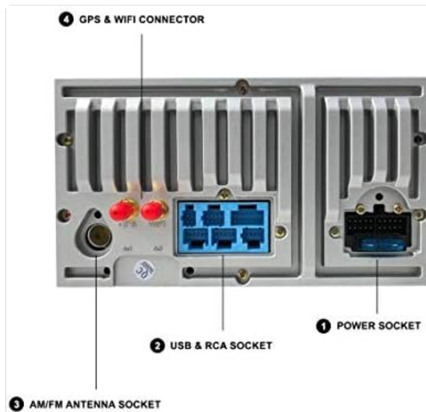
Figure 2: Rear Connection Ports. This image provides a detailed view of the rear panel of the Avison unit, highlighting its various connection ports. Clearly labeled are the Power Socket (1), USB & RCA Socket (2), AM/FM Antenna Socket (3), and GPS & WiFi Connector (4). These ports facilitate power supply, audio/video input/output, radio reception, and navigation/internet connectivity.
