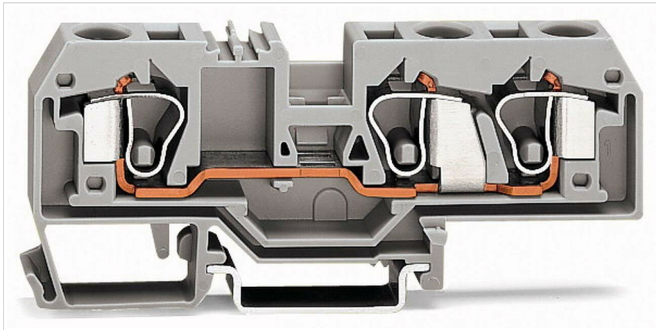
Figure 1: Cross-section view of the WAGO 284-681 3-Conductor Through Terminal Block, showing the internal spring clamp mechanism and conductor pathways. The grey housing encases the metallic current bar and the spring-loaded clamping units for secure wire termination.
