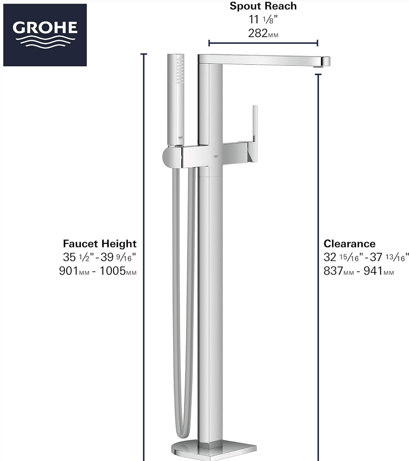
Image 2.1: Key dimensions of the GROHE Plus Floor Standing Tub Filler, including spout reach and overall height, important for planning installation.
