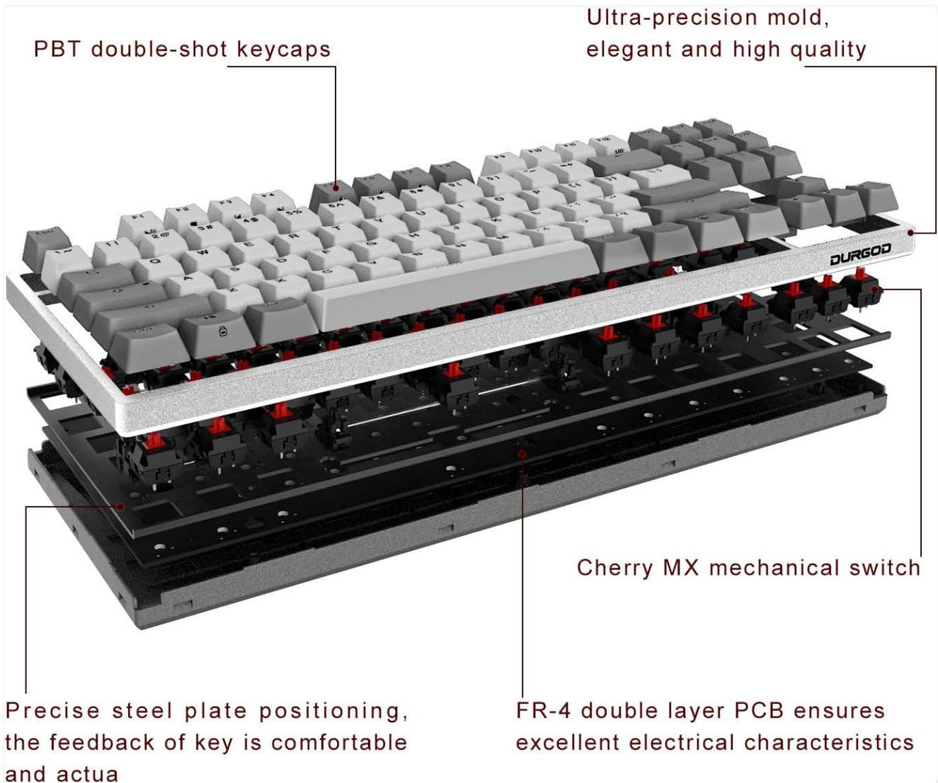
Image: An exploded diagram of the DURGOD K320 keyboard, illustrating its internal structure including PBT double-shot keycaps, Cherry MX mechanical switches, precise steel plate positioning, and FR-4 double layer PCB.
