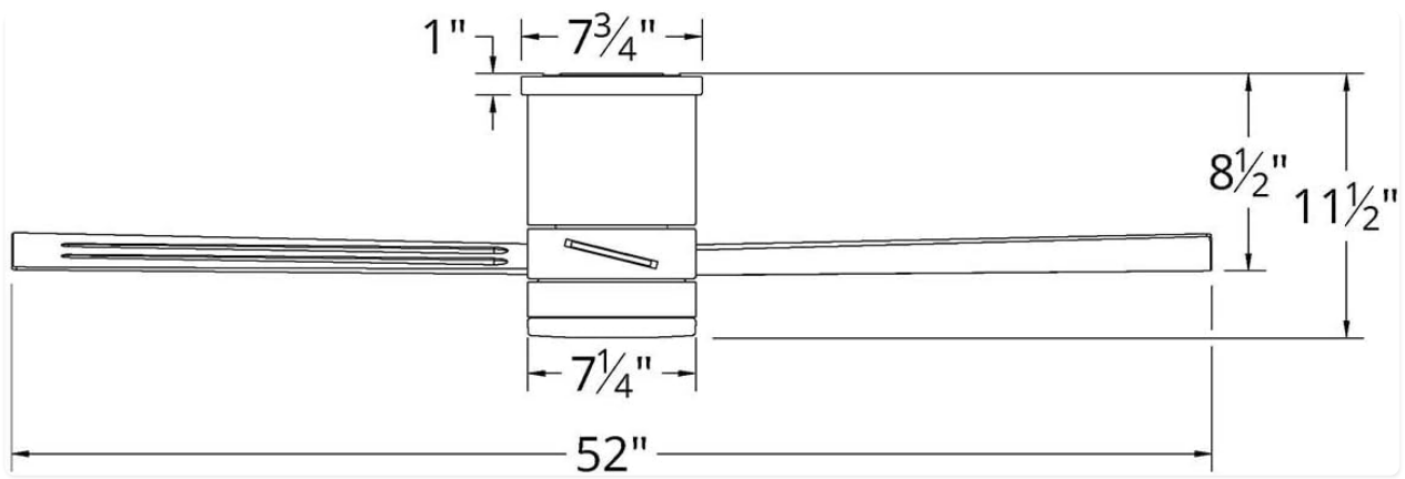
A detailed diagram illustrating the precise measurements of the Modern Forms Axis 52-inch Smart Ceiling Fan, including blade span, height, and motor housing dimensions.
