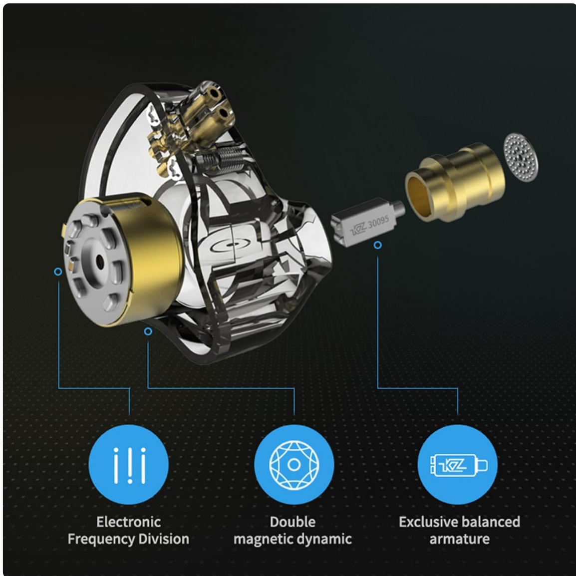
Image: An exploded view of the earphone's internal structure, highlighting the electronic frequency division, double magnetic dynamic driver, and exclusive balanced armature.
