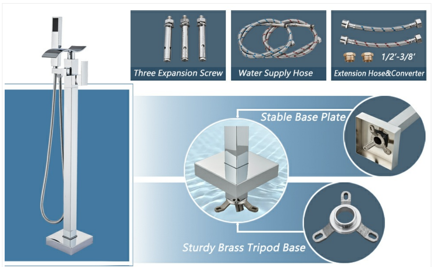
Image 5.1: Detailed view of the faucet's stable base design, including the tripod bracket and mounting screws.
