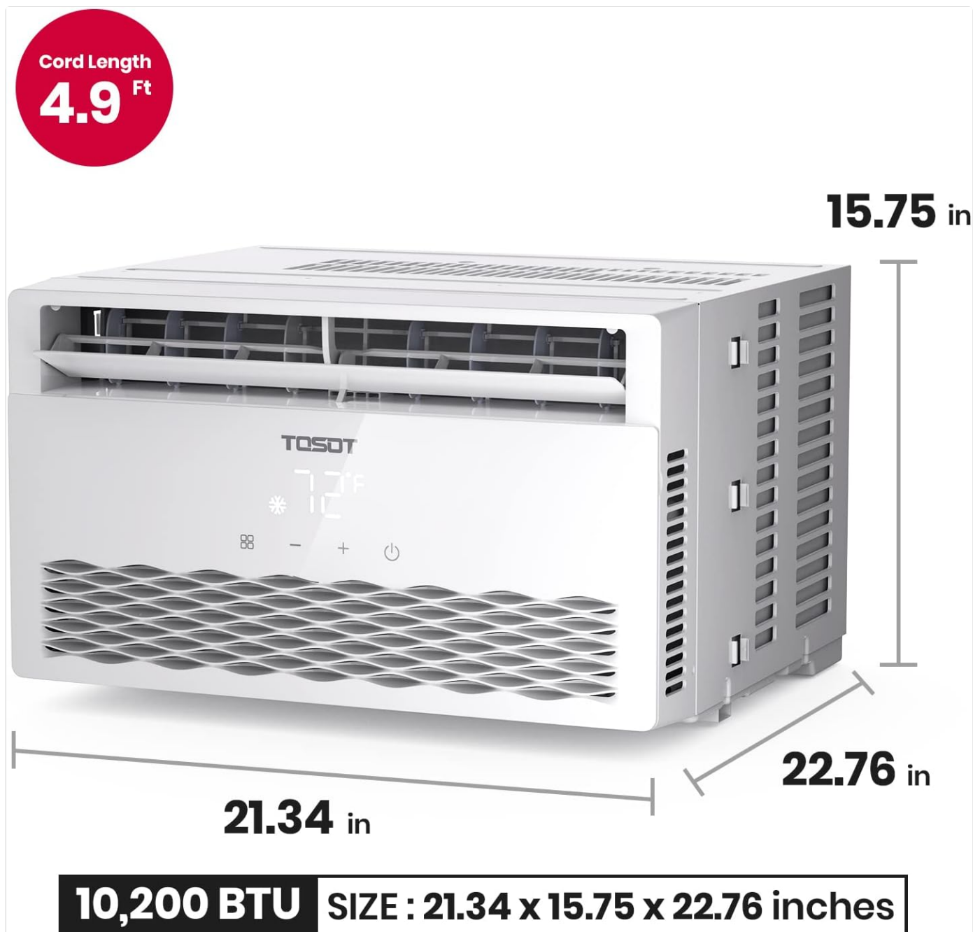
Figure 7.1: Product Dimensions. This image provides a visual representation of the air conditioner's physical dimensions and cord length.
