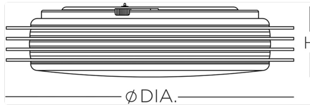
Figure 3.1: Dimensional diagram of the AFX Lenox LED Flush Mount Ceiling Light. This diagram illustrates the diameter (DIA) and height (H) of the fixture, which are approximately 23 inches and 3.37 inches respectively, aiding in pre-installation planning.
