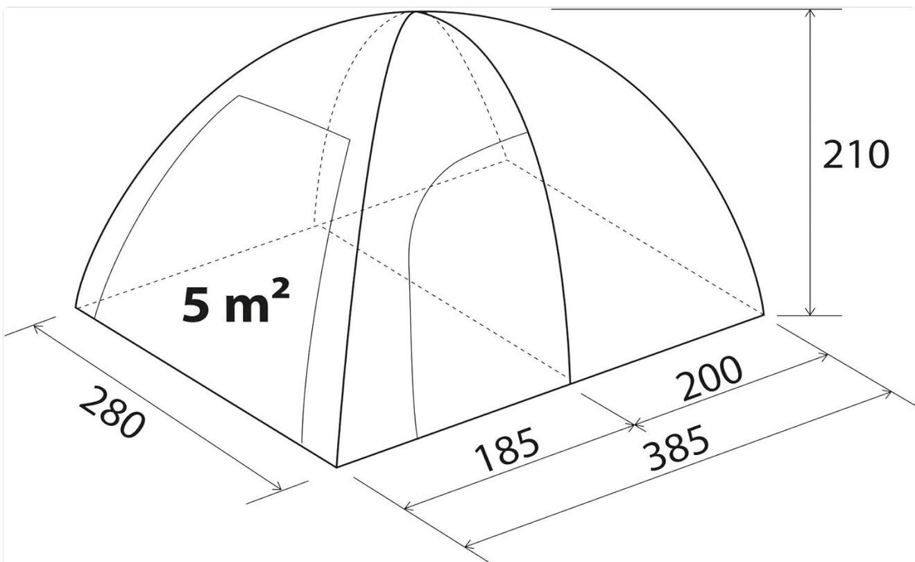
Figure 2.1: External dimensions of the tent, illustrating its footprint and height for planning your campsite layout. Dimensions are in centimeters.
