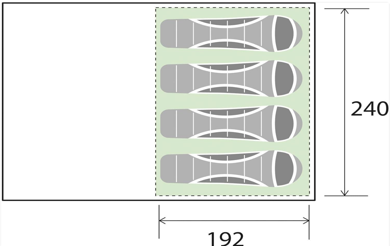
Figure 3.1: Internal layout of the sleeping area, demonstrating how four sleeping mats can be arranged comfortably within the tent's dimensions. Dimensions are in centimeters.
