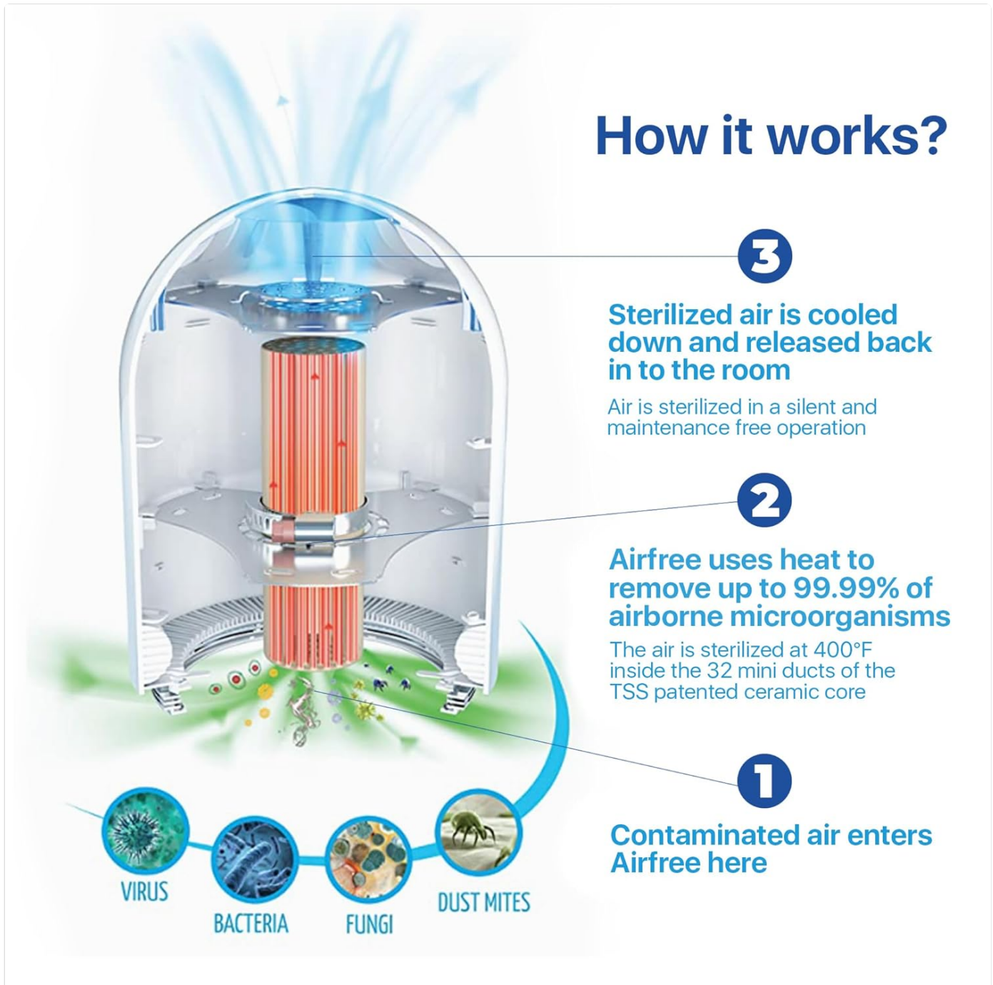
Figure 5: An internal diagram illustrating the Thermodynamic TSS Technology, showing how contaminated air is drawn in, sterilized by heat, and then released as clean air.
