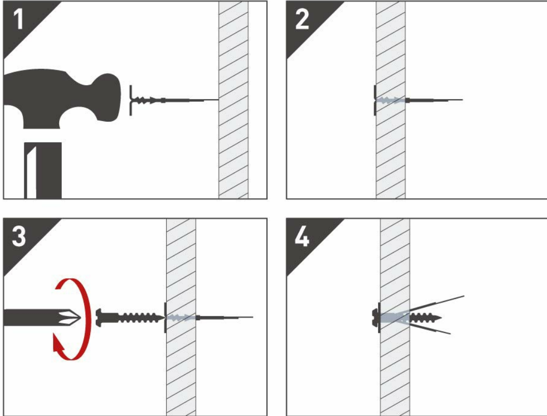
Figure 6: Hammering Drywall Anchors.
