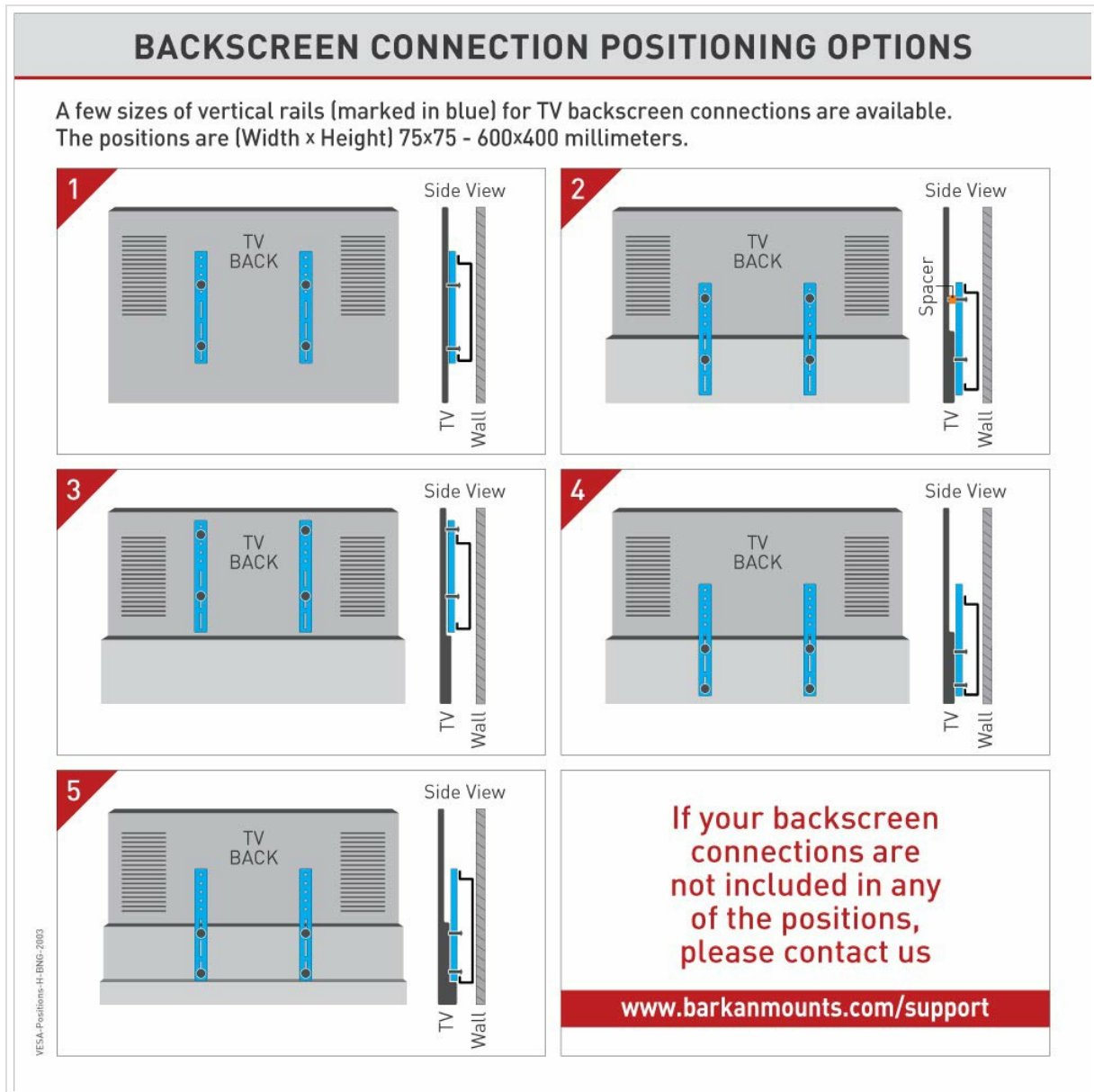
Figure 10: Backscreen Connection Positioning Options.
