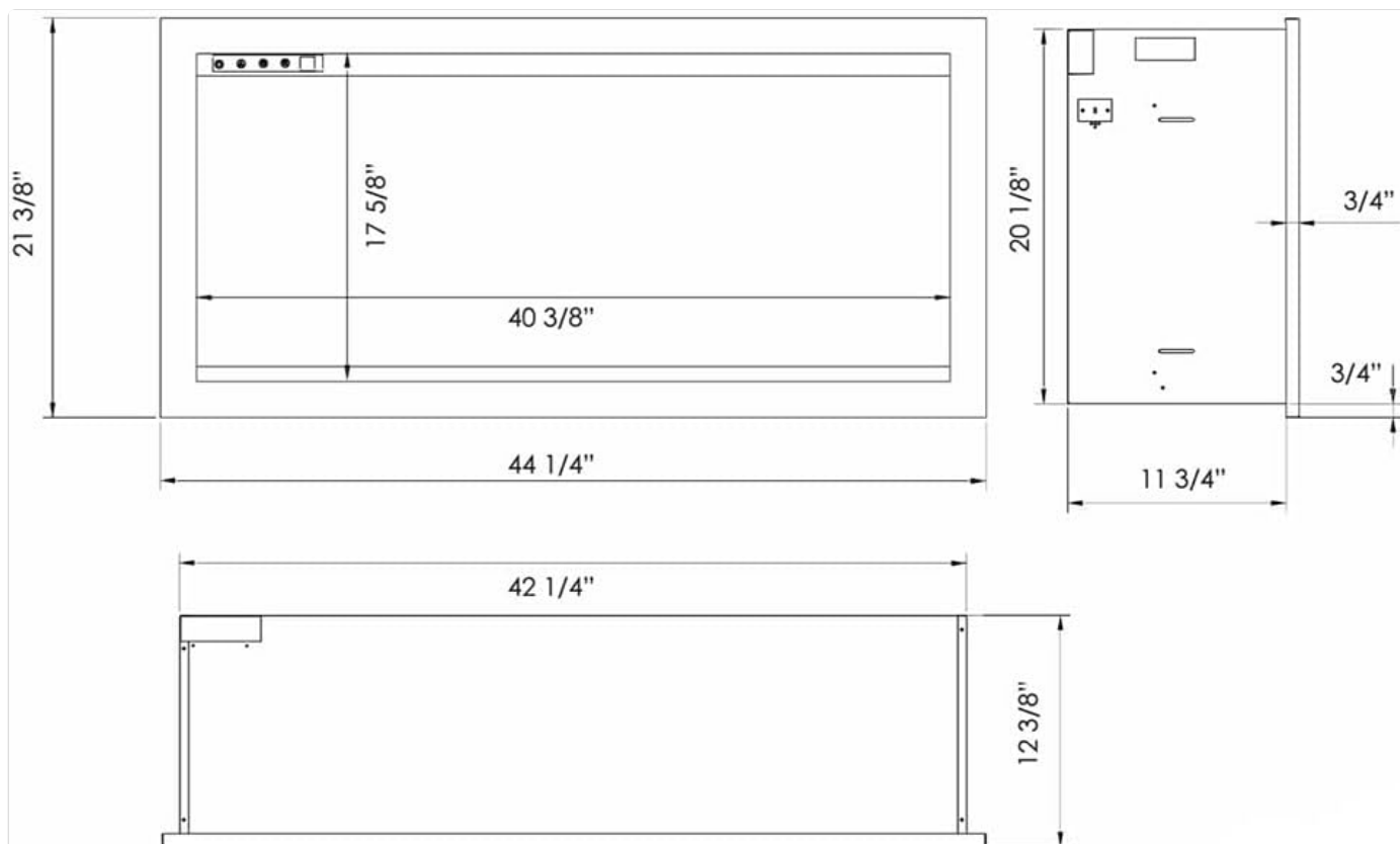
Figure 4.1: Technical drawing illustrating the precise dimensions and cutout requirements for installation.
