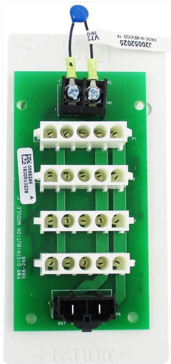
Figure 2: Internal view of the Simplex 4100-0634 module's circuit board, highlighting the arrangement of the terminal blocks and internal wiring for power distribution.
