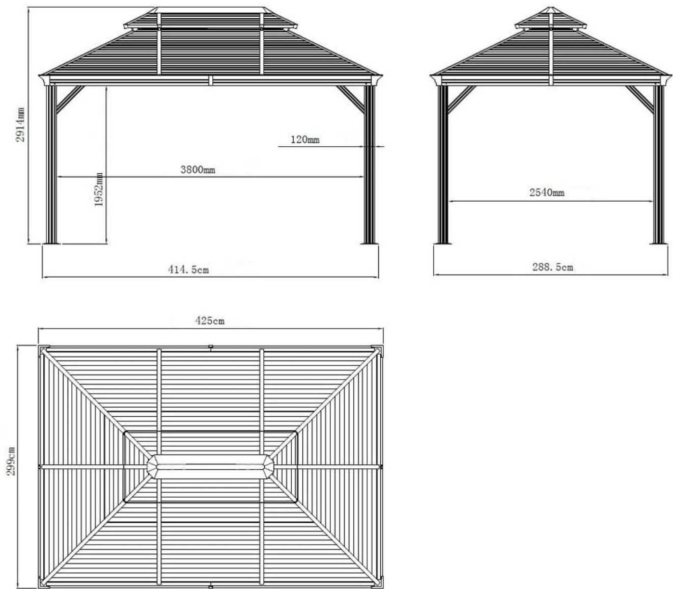
Figure 2: Technical drawing illustrating the dimensions and structure of the gazebo.
