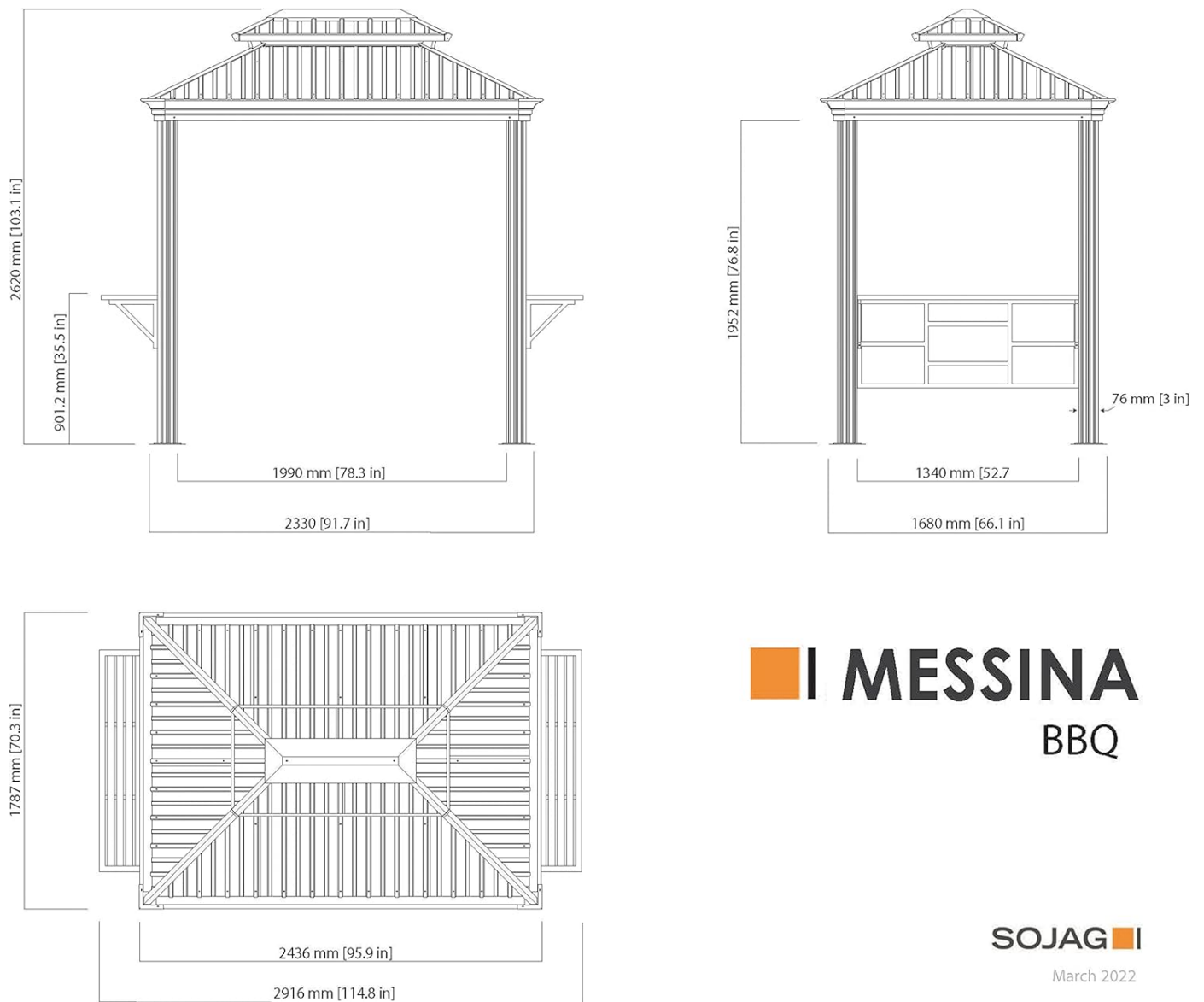
Image: Detailed dimensions and structural overview of the Messina Grill Gazebo.
