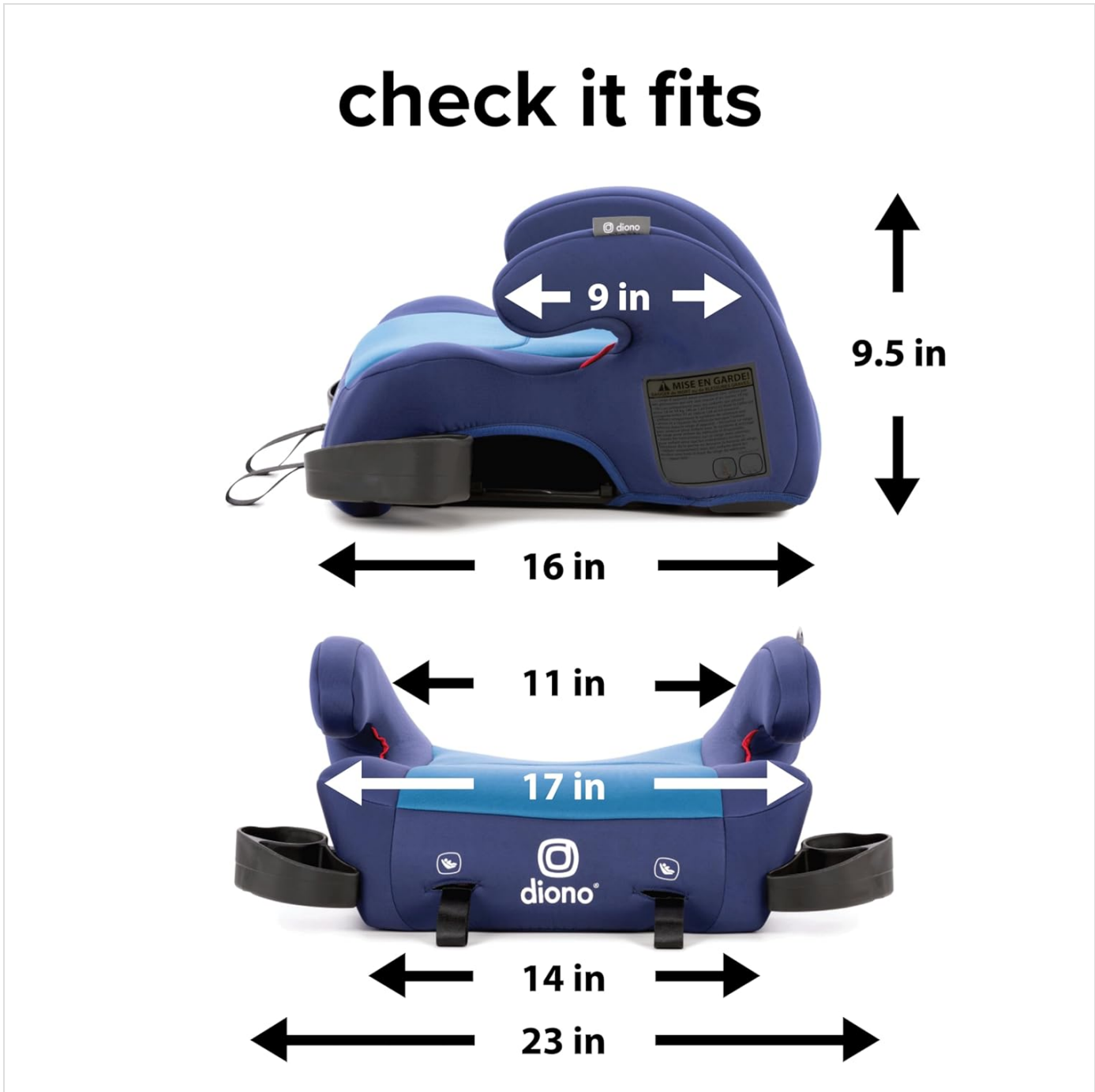
Image: A diagram showing the key dimensions of the Diono Solana 2 XL booster seat, including width, depth, and height measurements for proper fit in a vehicle.
