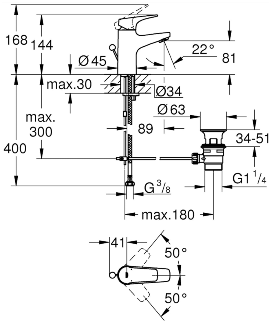
Image: Technical diagram illustrating the dimensions and installation requirements for the GROHE Start Flow faucet, including connections and pop-up waste mechanism.
