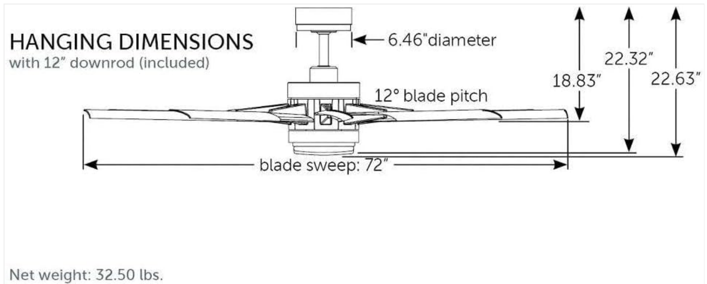
Image: Diagram showing the hanging dimensions of the Fanimation Odyn Custom 72-inch fan, including the 12-inch downrod, 6.46-inch diameter canopy, and 22.63-inch total height.
