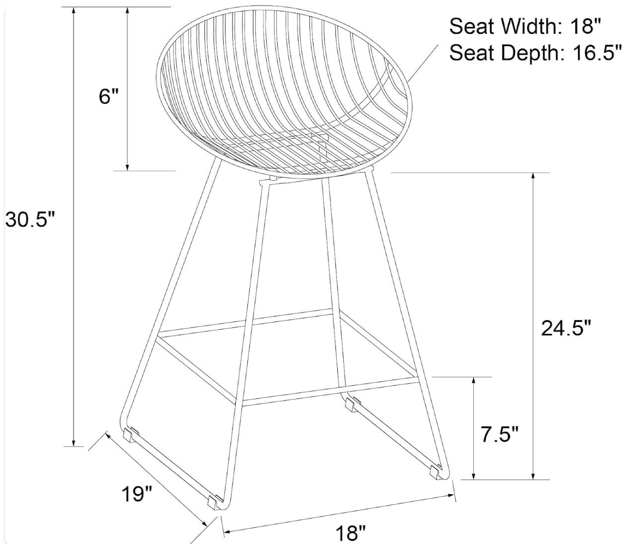
Image: Technical drawing illustrating the dimensions of the CosmoLiving Ellis Barstool.
