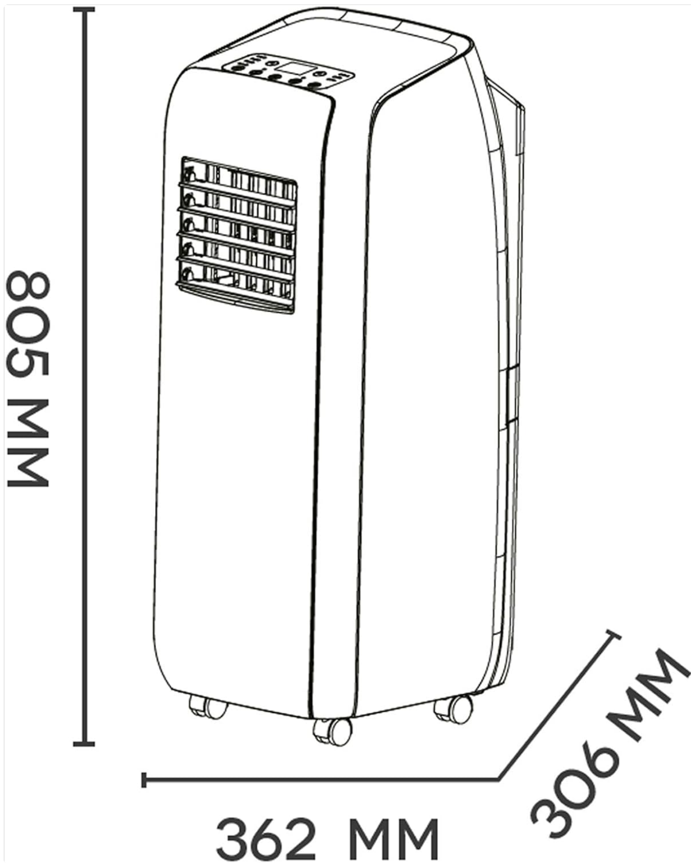
Figure 6: Dimensions of the unit.
