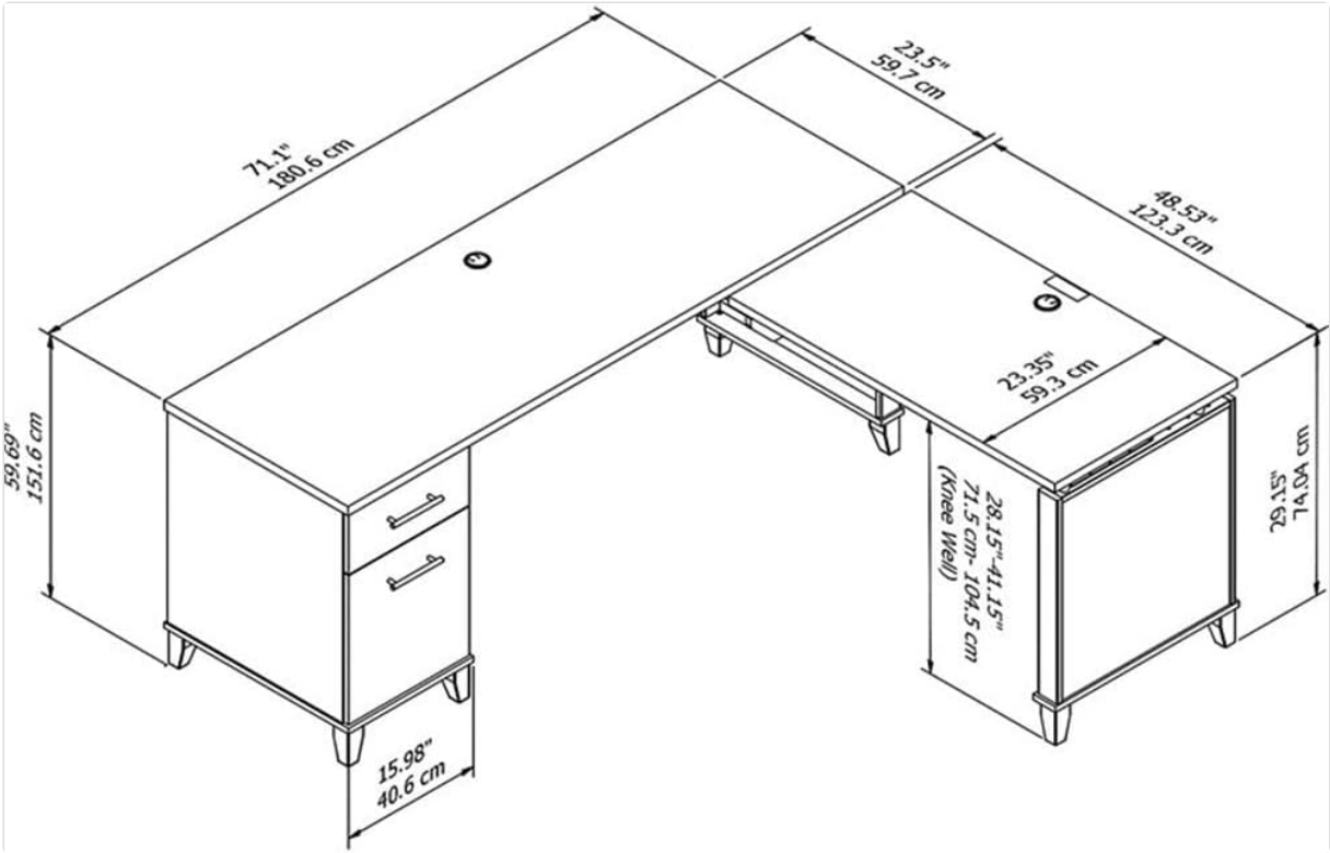
Image 7.1: Technical diagram displaying the overall dimensions of the L Shaped Desk in both inches and centimeters.
