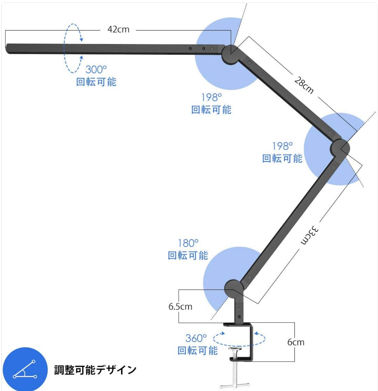
Figure 4: The lamp features a highly adjustable design, allowing for precise positioning of light with multiple pivot points.
