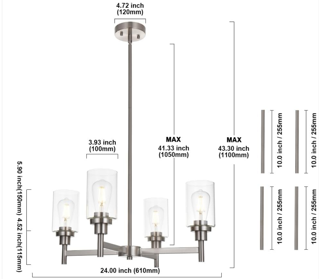
Image: Detailed diagram showing the dimensions of the VINLUZ 4 Light Modern Chandelier, including length, width, height, and rod lengths.
