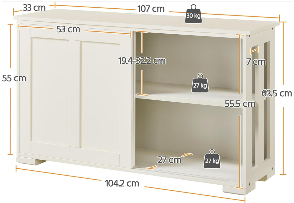
Image: Diagram showing the overall dimensions of the cabinet (107 cm length, 33 cm depth, 63.5 cm height) and internal shelf dimensions, along with weight capacities for the top (30 kg) and shelves (27 kg each).
