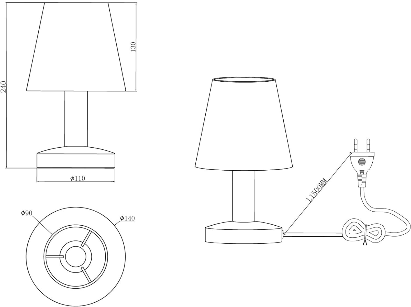
Figure 6: Technical diagram of the lamp, including cord length (L1500MM).
