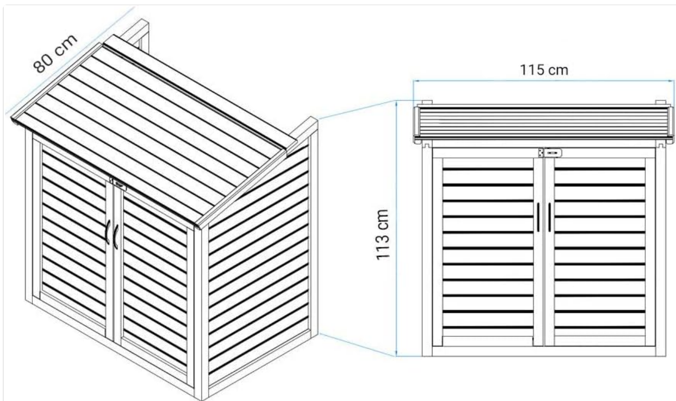
Figure 7.1: Dimensional diagram of the Interline Bali Filter Housing.
