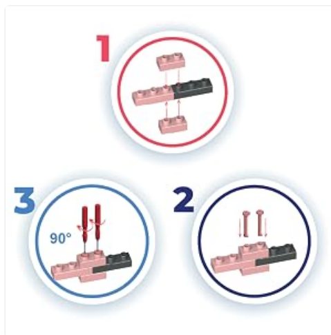
Image: Detailed three-step diagram for JEKCA block assembly. Step 1 shows two blocks being connected. Step 2 shows pins being inserted. Step 3 shows the pin driver turning the pins 90 degrees to secure them.
