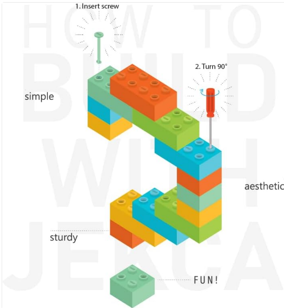
Figure 2: Illustration of the JEKCA interlocking pin system.
