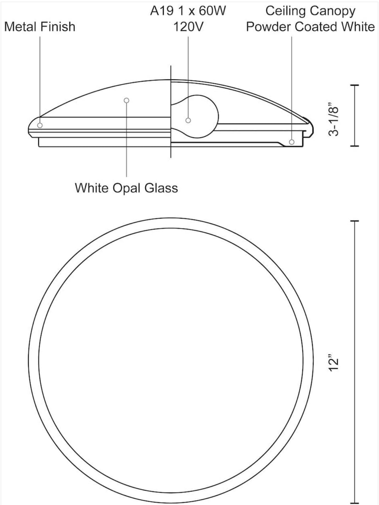
Image 4.1: Technical diagram illustrating the fixture's components and assembly points.
