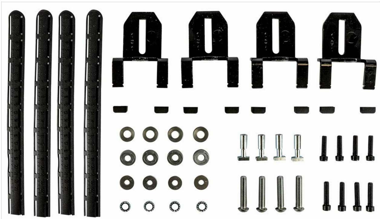
Figure 1: Example of a MENABO roof rack foot, showing the attachment point and rubber pad for secure fitment.
