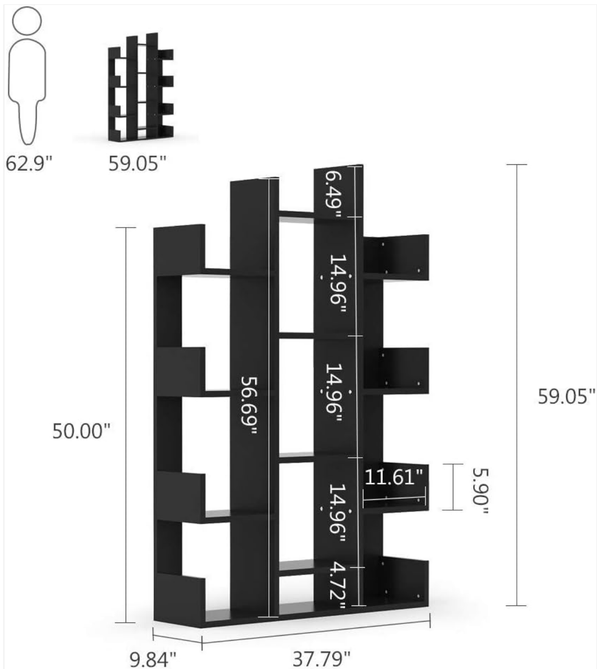
Image 6.1: Detailed dimensional drawing of the bookcase, including overall and individual shelf measurements.
