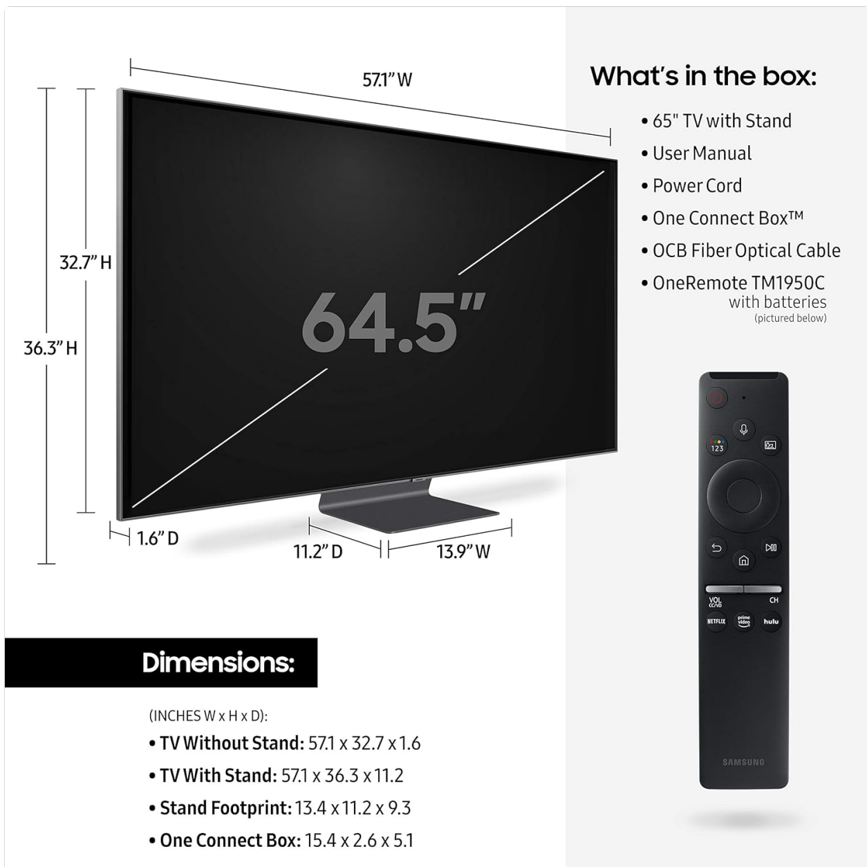
Figure 2.1: Detailed dimensions of the Samsung Q90 Series TV, including width, height, and depth with and without the stand, along with the screen diagonal measurement.
