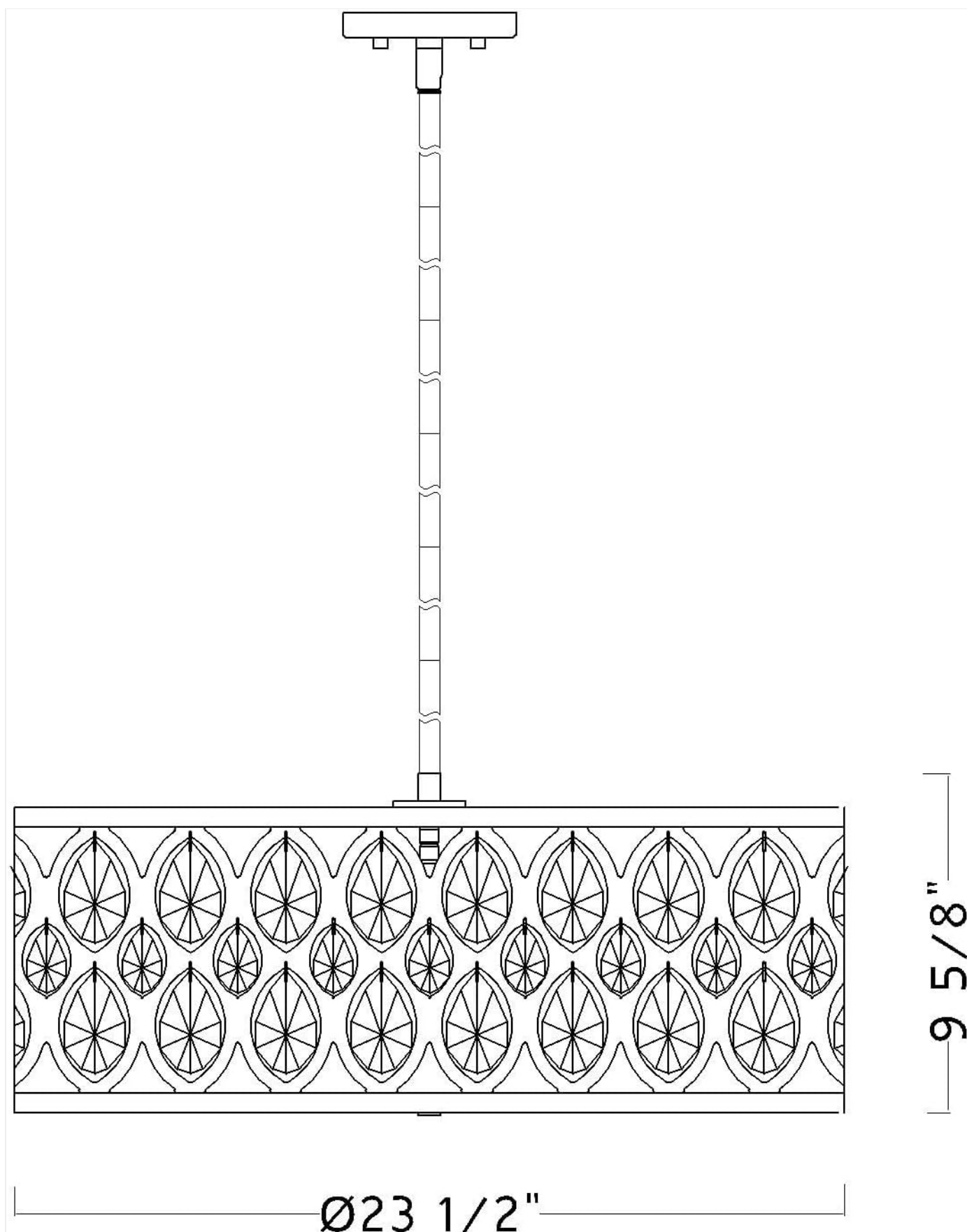
Image: Technical line drawing illustrating the chandelier's dimensions (23 1/2" diameter, 9 5/8" height) and general mounting structure.
