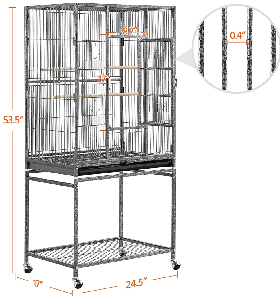
Figure 2: Detailed dimensions of the bird cage (24.5"L x 17.0"W x 53.5"H).
