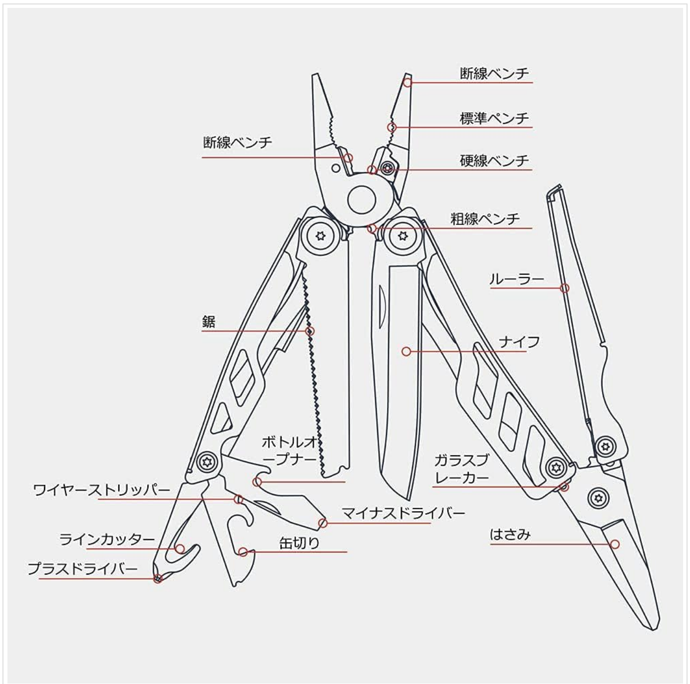
Image 3.2: Diagram illustrating all 16 tools integrated into the multi-tool.
