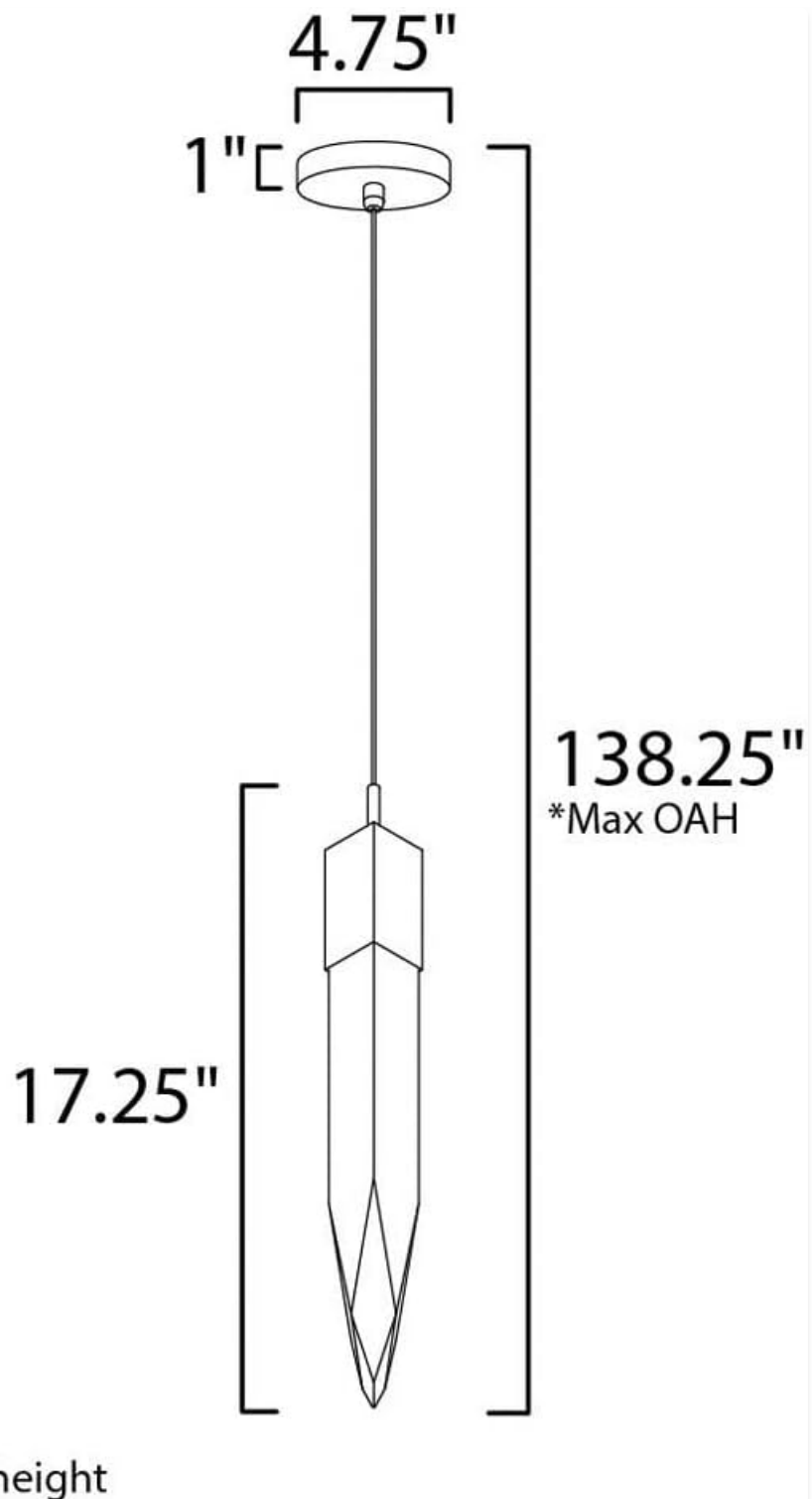
Figure 4.1: Dimensional diagram of the pendant light, indicating a 4.75-inch diameter canopy and a 17.25-inch fixture height, with a maximum overall height of 138.25 inches.
