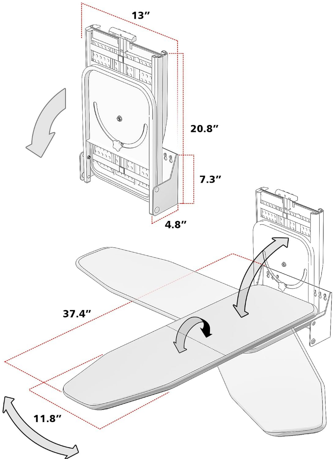
Figure 1: Product dimensions and swivel mechanism. The board measures 37.4"L x 11.8"W when open. When folded, it measures 13"L x 4.8"W x 20.8"H.
