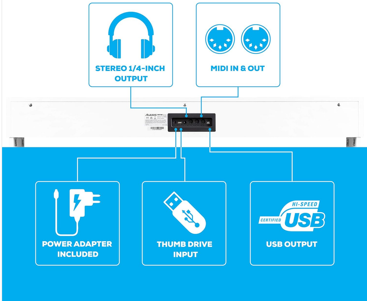
Image 2: Rear panel connections of the Alesis Virtue AHP-1W, including Stereo 1/4-inch Output, MIDI In & Out, Power Adapter input, Thumb Drive input, and USB Output.
